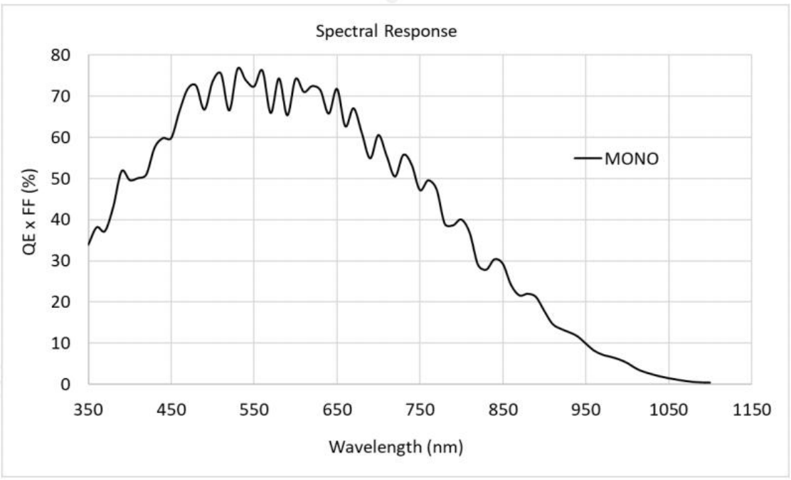
Figure 8 – Spectral response characteristic for MONO sensor
